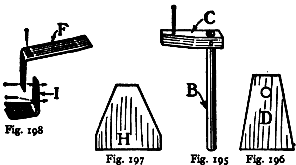
FIGS. 195-198. — Details of Interrupter.
